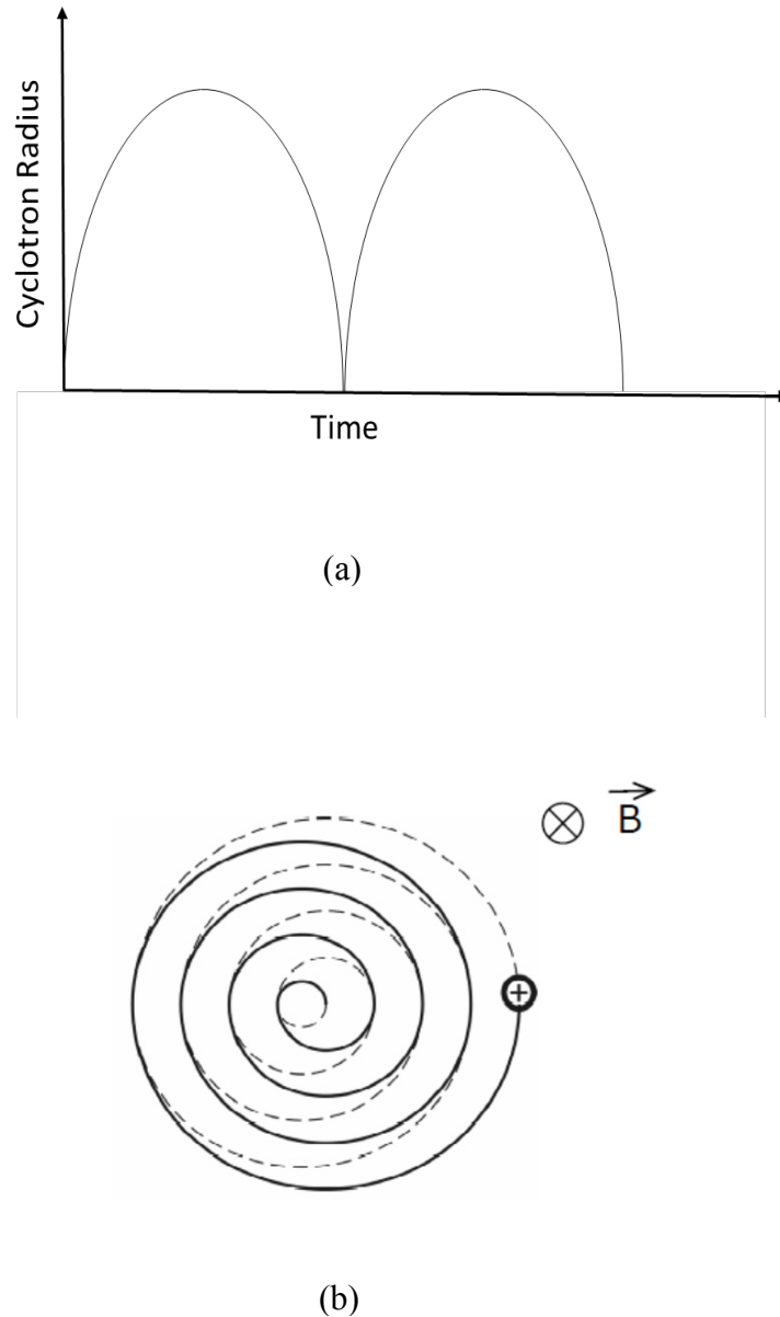
Figure 2.6 (a) Change in ion cyclotron radius (b) ion x-y trajectory as ions excite and de-excite due to difference between the excitation frequency and ion cyclotron frequency in SORI-CID. (Adapted with permission from “Stored waveform inverse Fourier transform (SWIFT) ion excitation in trapped-ion mass spectrometry: Theory and applications” by Guan SH and Marshal AG, 1996, Int. J. Mass Spectrom. Ion Processes , 5-37. copyright (1996) Elsevier Science B.V.)
